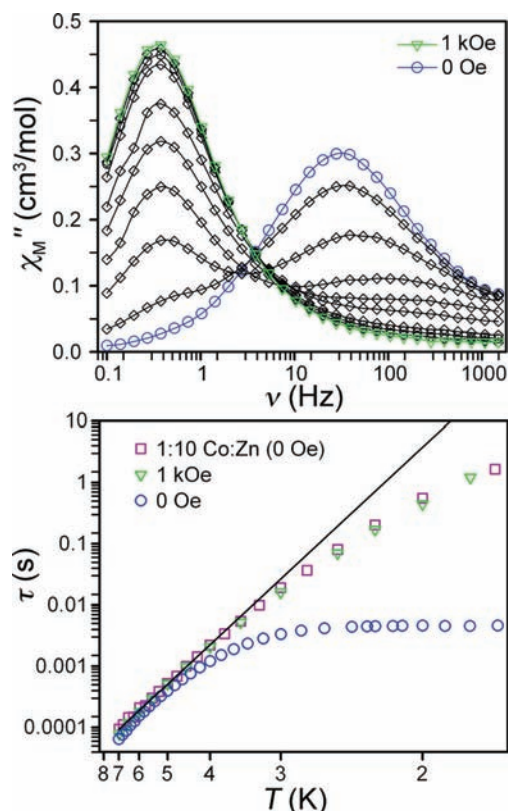
Figure 3. Top: Molar out-of-phase ac susceptibility ( \chi_M'' ) collected on pure 1 at 2 K under applied dc fields from 0 to 1 kOe in 100 Oe increments. Solid lines are guides for the eye. Bottom: Arrhenius plots of relaxation times of 1 as a pure substance under 0 and 1 kOe, and diluted in a matrix of (\text{Ph}_4\text{P})_2[\text{Zn}(\text{SPh})_4] under 0 Oe. The black line corresponds to a linear fit to the highest-temperature data of the diluted sample, as described in the main text.
